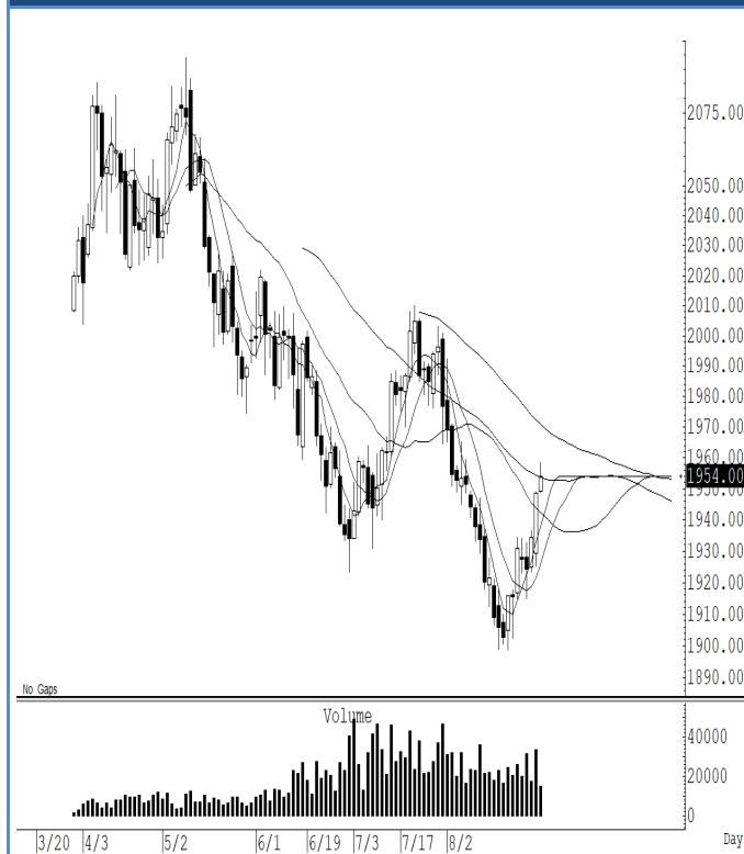
GOU23 (Close 1,954.00 Chg 6.50)
